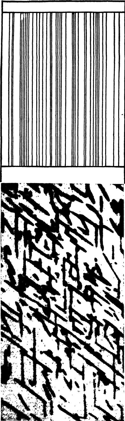
FIG. 9.—Regular spacing of segregate structures of Widmanstätten type.
